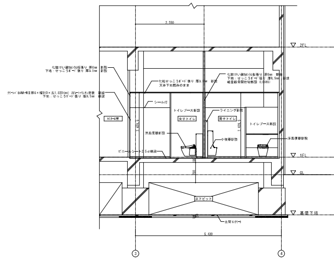
短計図(改修) S:1/50
